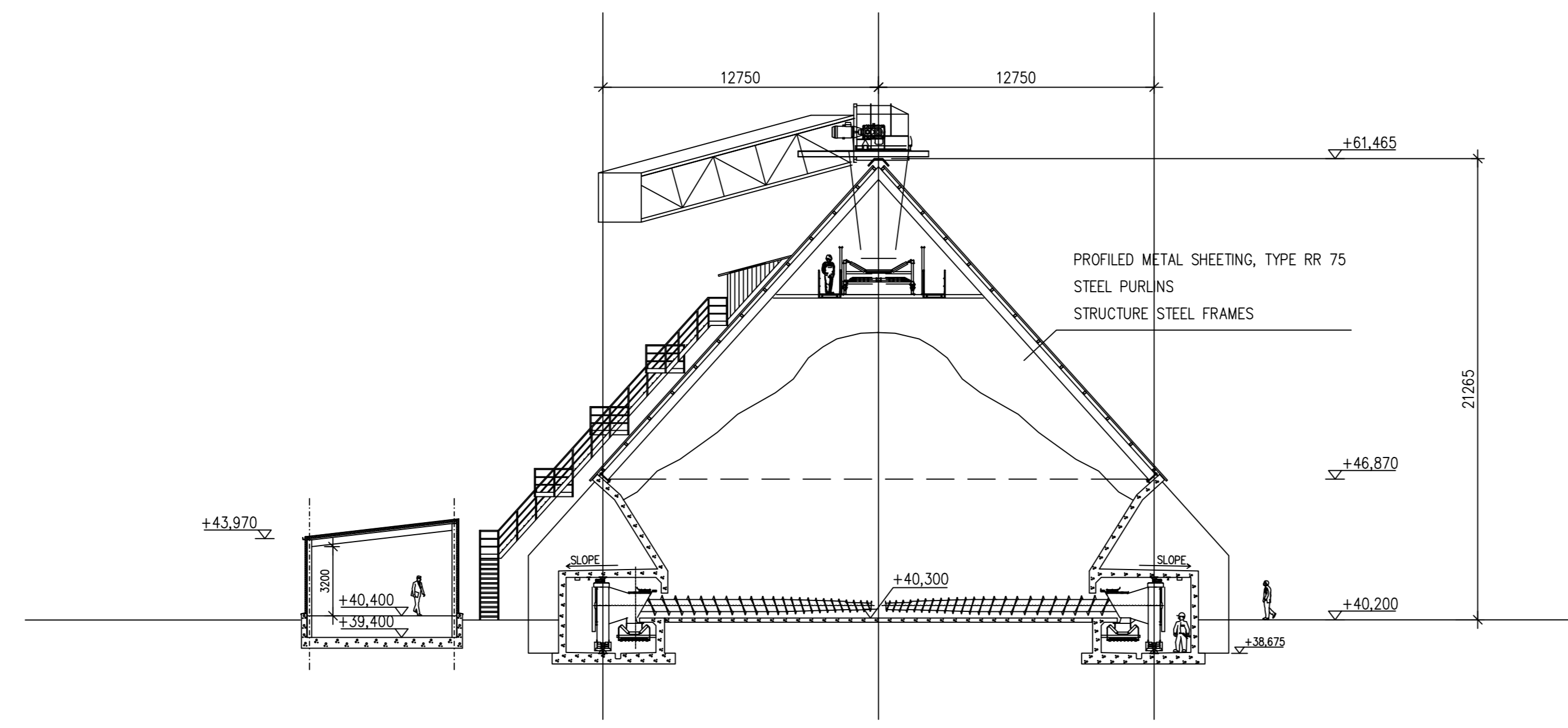
SECTION A-A [REFER TO DRG. QS-000206-01-D460-040]
